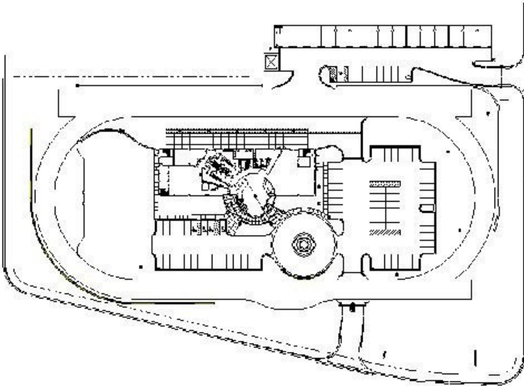
Second Floor Plan: Upper Atrium and Pre-function Area (center), Theatre (center left), Dining, Kitchen, and Group Meeting Rooms (upper left), Private Meeting Rooms and Board Room (bottom left), Outdoor Balcony (top), and Corporate Offices
